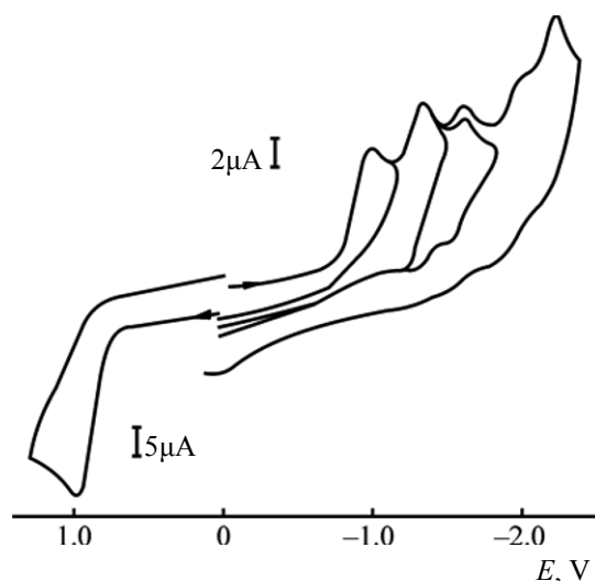
Fig. 2. Cyclic voltammograms of nickel complex XVIII ; concentration 10 -3 M, glassy carbon electrode, DMF, Bu 4 NClO 4 .
